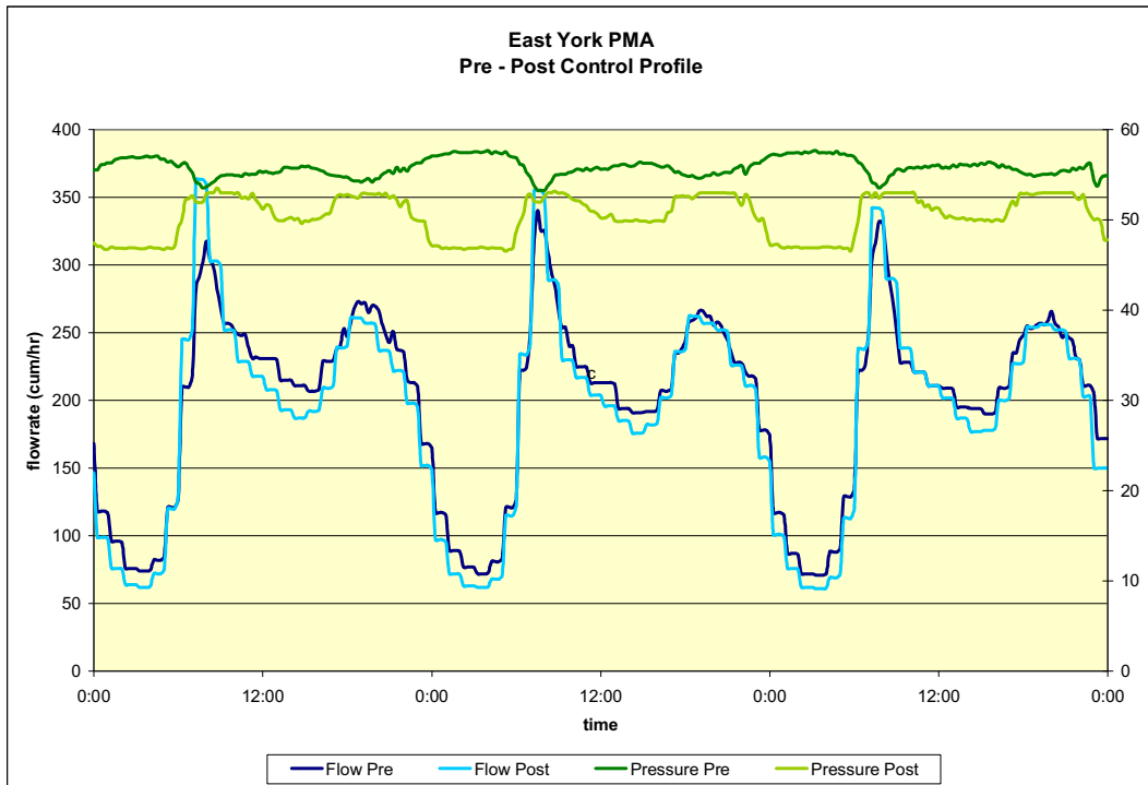
Figure 7 - No-Control vs. Control PMA Flow & Pressure Profile
