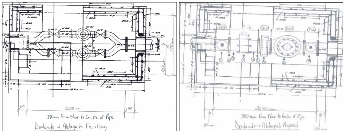
Figure 4 - Donlands & Aldwych - Existing & Proposed Chamber Configuration
