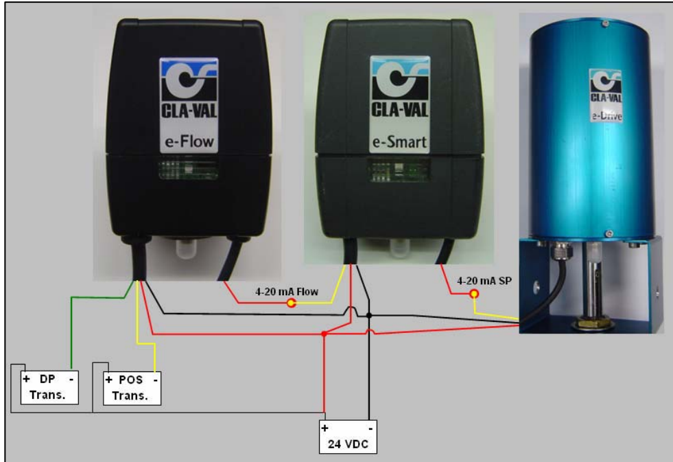
Figure 3 - Cla-Val Flow Modulation Controller Wiring
