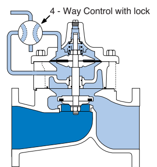
Modulating Action
