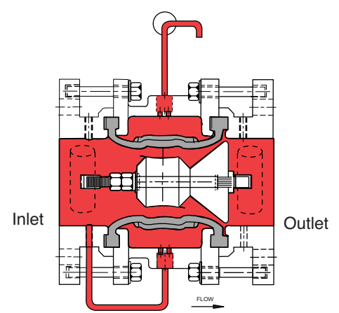
Modulating Action
