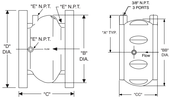
Flanged Style 6", 8", 10", & 12" sizes
