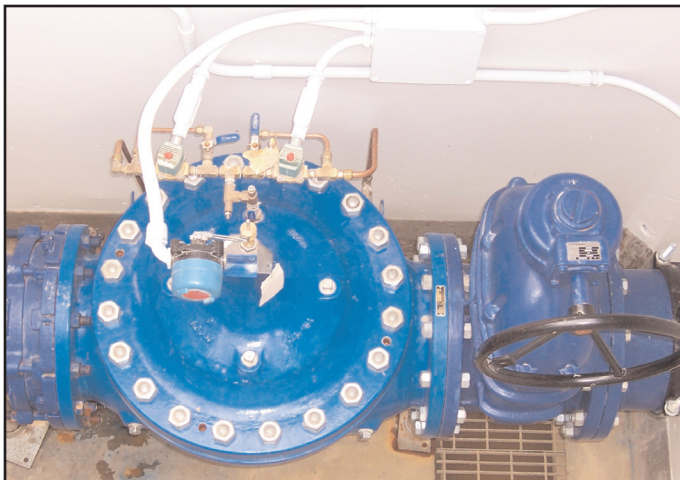
Typical Application Cla-Val Blending Valves
