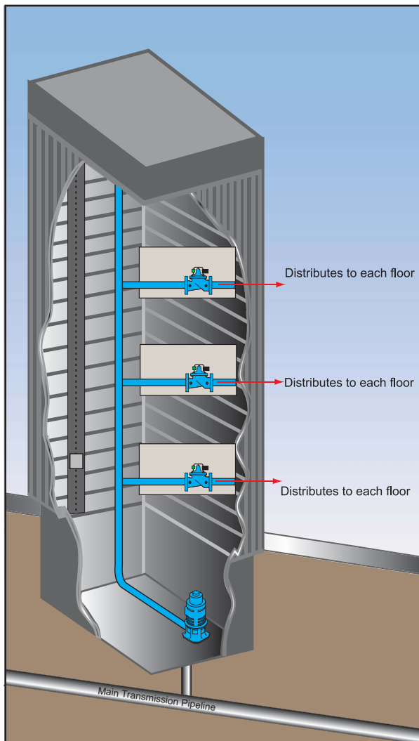
Domestic Water Systems in High-Rise Buildings -- Pressure Reducing Valve Stations
