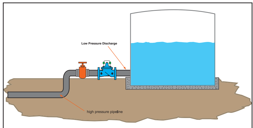
Ground Storage Tank Fill Valves
