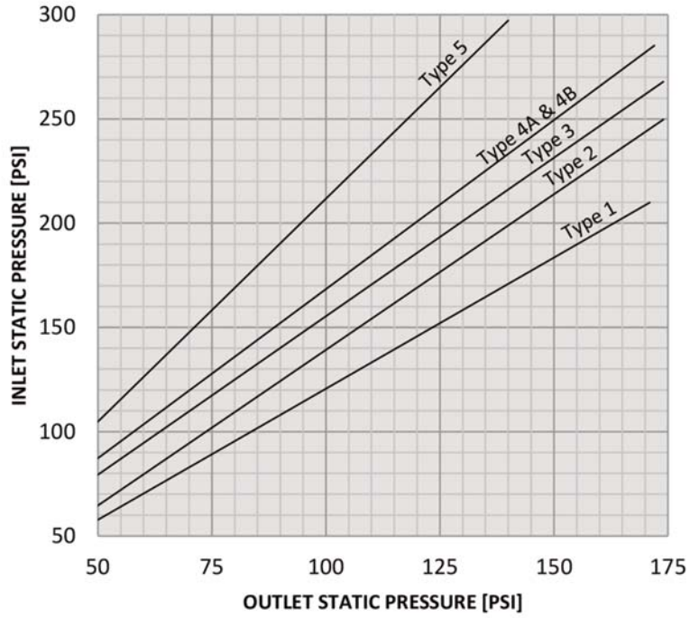
1.5" 90-FS-PRV-25 Angle Body Inlet vs. Outlet Pressure @ Static Flow
