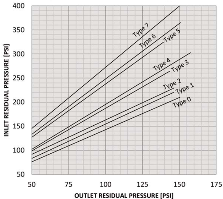
2.5" 90-FS-PRV-25 Inline Body Inlet vs. Outlet Pressure @ 50-200 [GPM]
