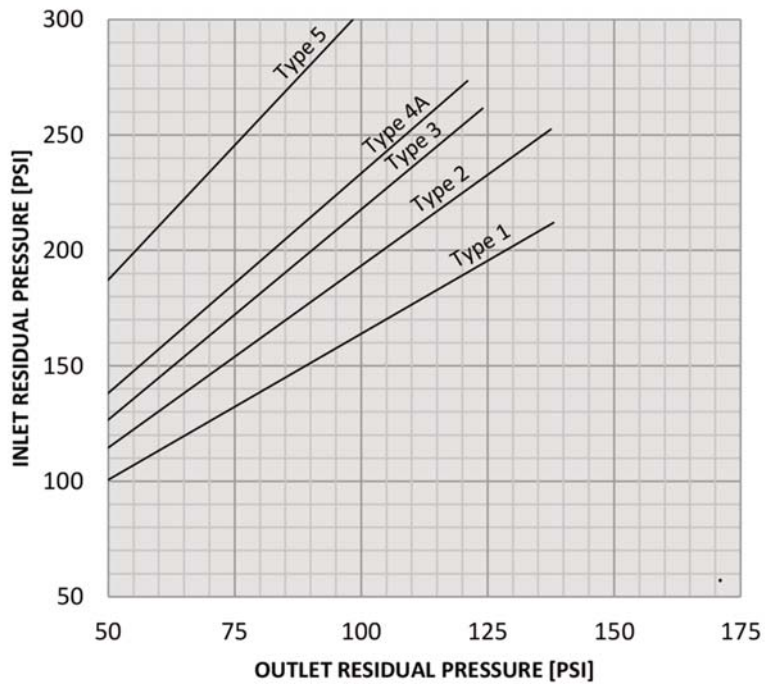
1.5" 90-FS-PRV-25 Angle Body Inlet vs. Outlet Pressure @ 200-250 [GPM]
