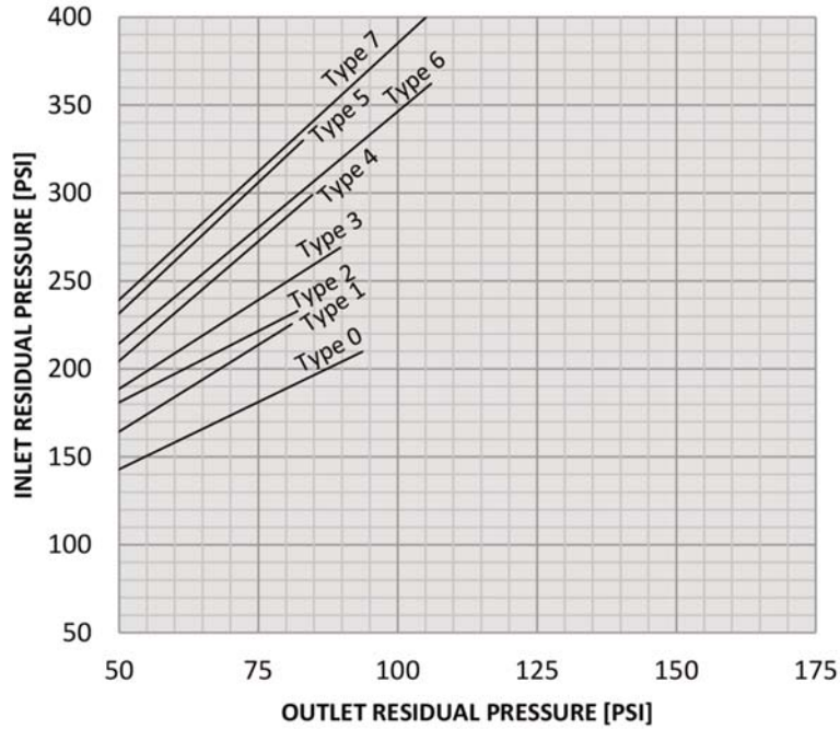
2.5" 90-FS-PRV-25 inline Body Inlet vs. Outlet Pressure @ 400-500 [GPM]
