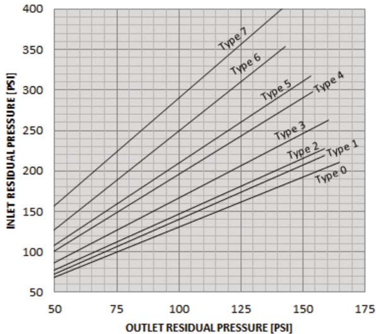
2.5" 90-FS-PRV-25 Angle Body Inlet vs. Outlet Pressure @ 200-300 [GPM]
