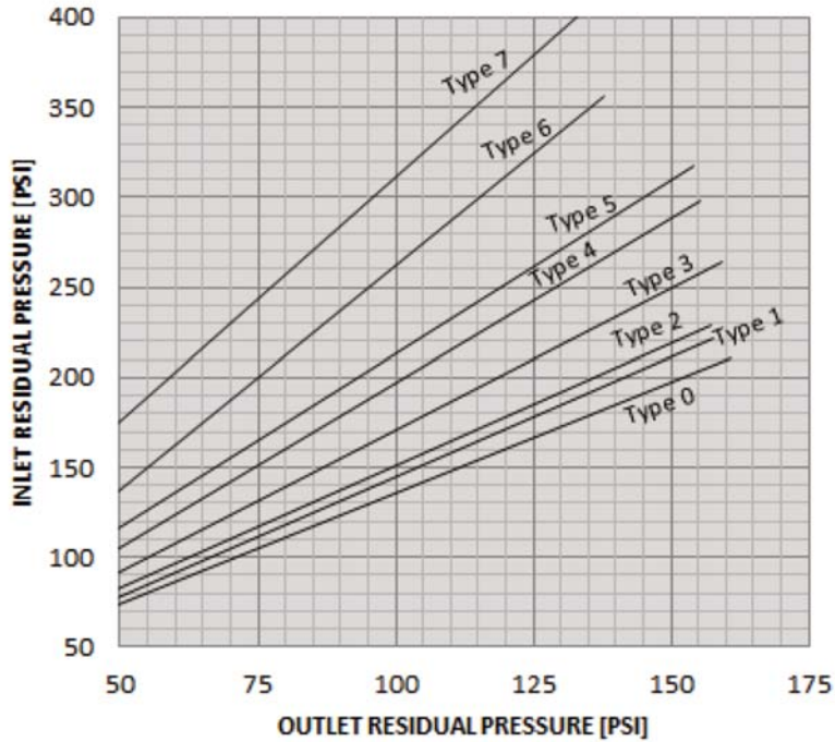
2.5" 90-FS-PRV-25 Angle Body Inlet vs. Outlet Pressure @ 300-400 [GPM]
