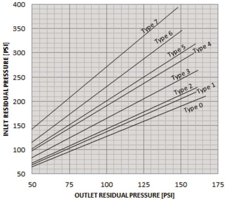
2.5" 90-FS-PRV-25 Angle Body Inlet vs. Outlet Pressure @ 50-200 [GPM]
