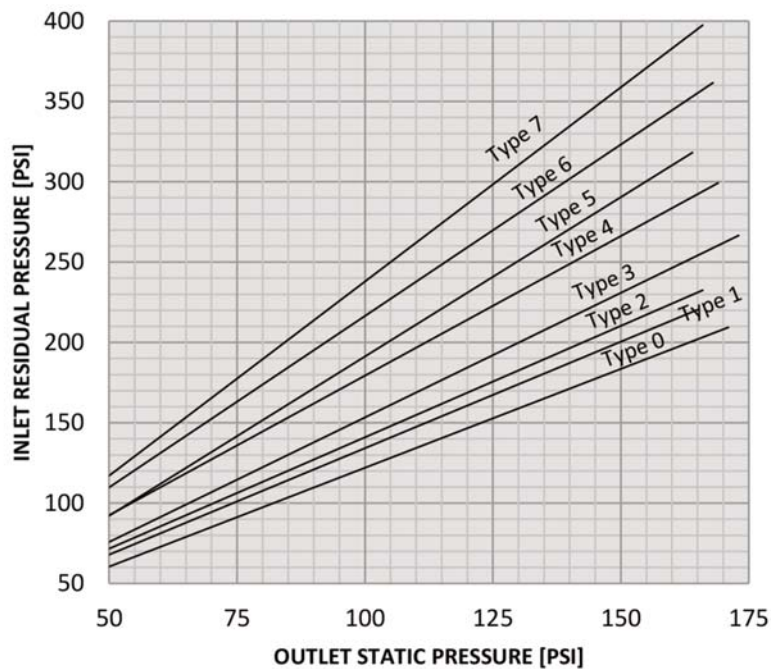
2.5" 90-FS-PRV-25 Inline Body Inlet vs. Outlet Pressure @ Static Flow
