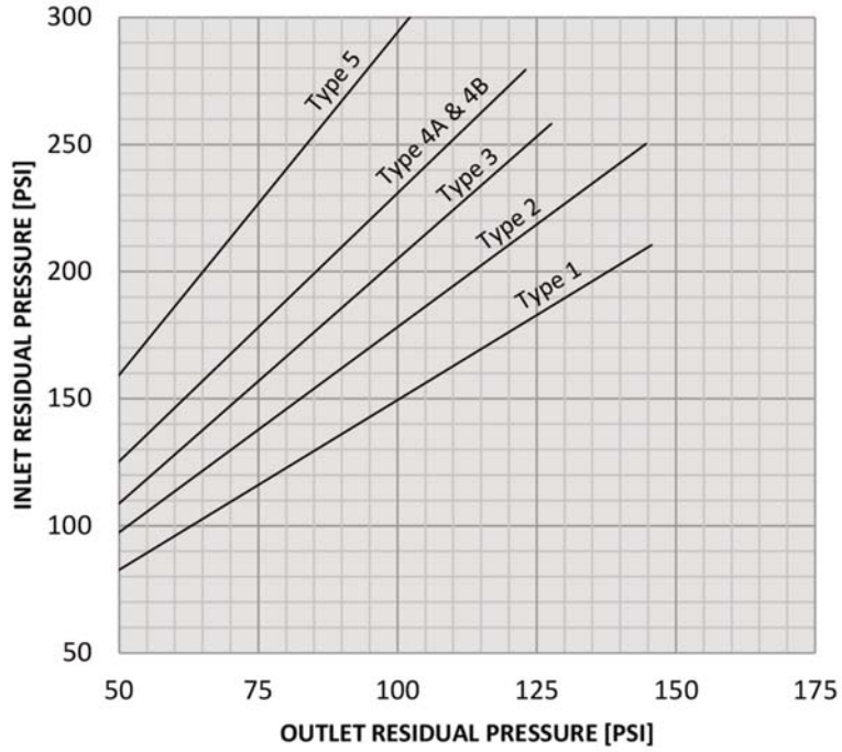
1.5" 90-FS-PRV-25 Angle Body Inlet vs. Outlet Pressure @ 50-200 [GPM]
