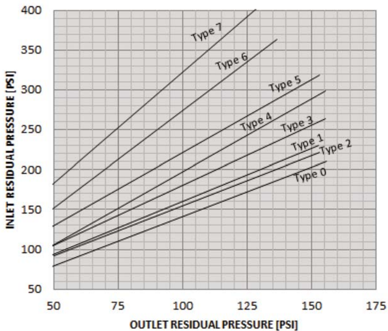
2.5" 90-FS-PRV-25 Angle Body Inlet vs. Outlet Pressure @ 400-500 [GPM]
