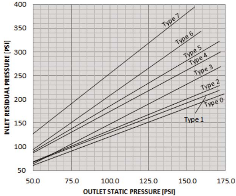
2.5" 90-FS-PRV-25 Angle Body Inlet vs. Outlet Pressure @ Static Flow
