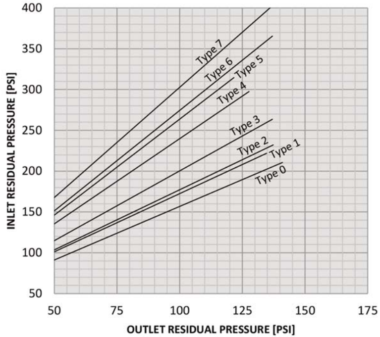
2.5" 90-FS-PRV-25 Inline Body Inlet vs. Outlet Pressure @ 300-400 [GPM]
