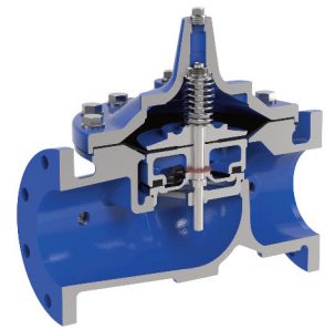
Model 100-01 Full Port Hytrol Main Valve
