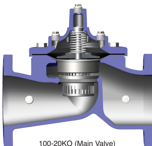
100-20KO (Main Valve)
