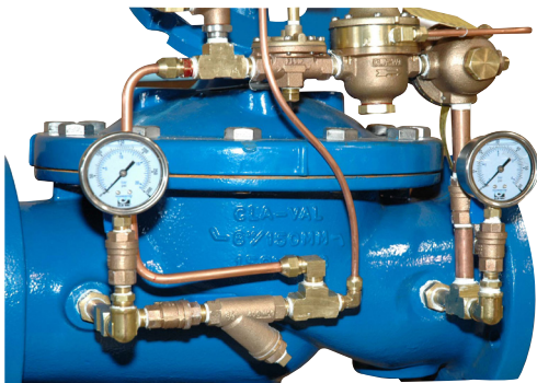
X141 both Gauges installed
